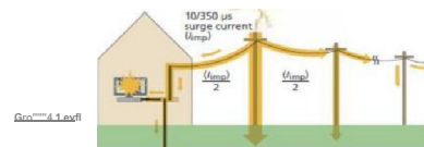
Figure 4: Illustration of lightning current flow from a direct strike to a nearby service (Source 1)
